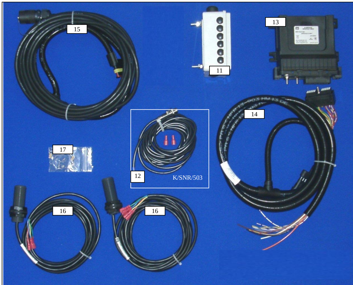
Single/Dual Motor Drive - HBM related components
